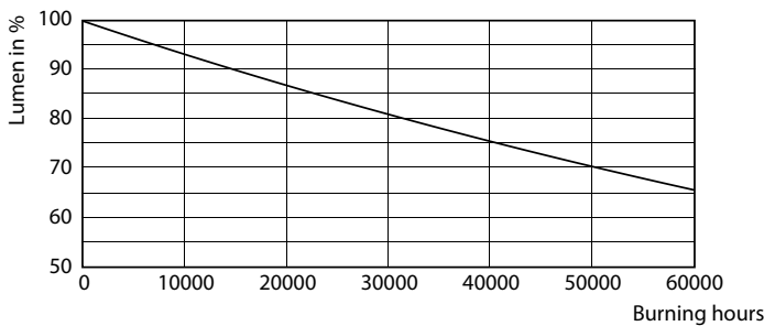
HIB NAM Trueforce 38W E39 Clear 727 36D ND
